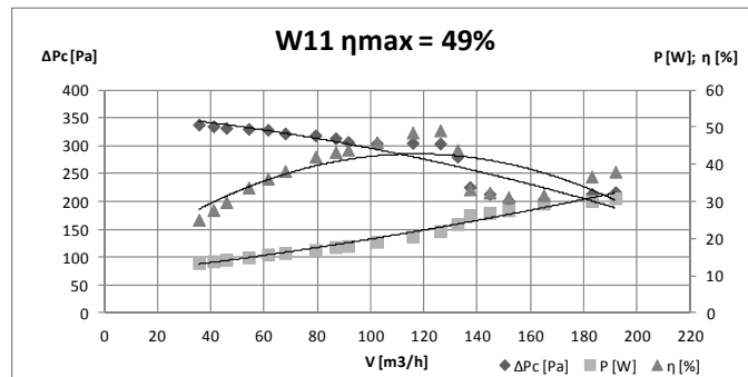
Fig. 12. Characteristics of fan W11
