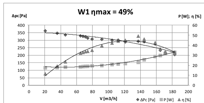
Fig. 2. Characteristics of fan W1
