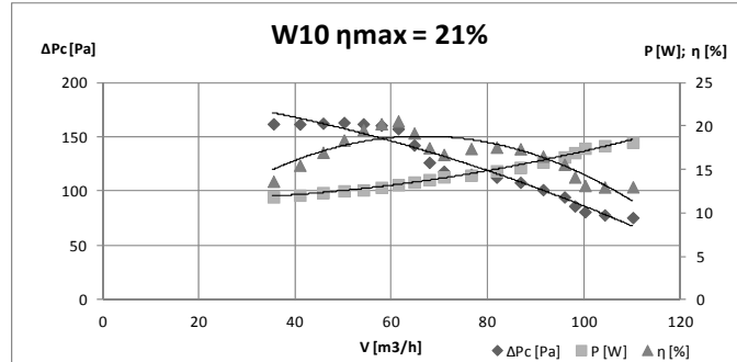
Fig. 11. Characteristics of fan W10
