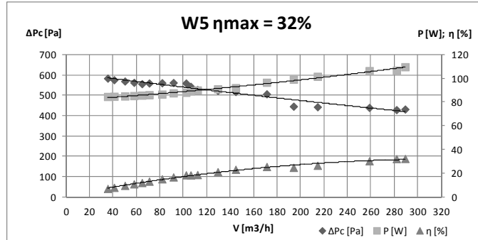
Fig. 6. Characteristics of fan W5
