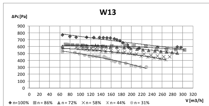
Fig. 14. Characteristics \Delta P_c for fan W13
