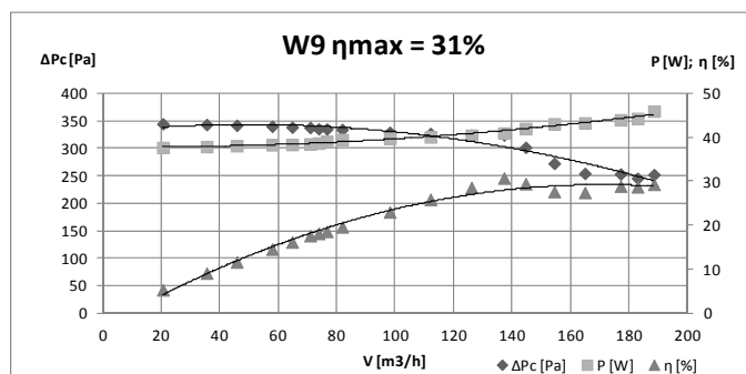
Fig. 10. Characteristics of fan W9
