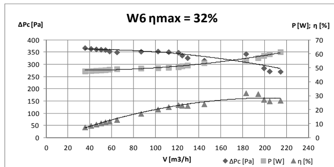
Fig. 7. Characteristics of fan W6
