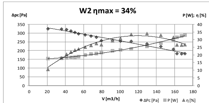
Fig. 3. Characteristics of fan W2
