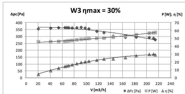
Fig. 4. Characteristics of fan W3
