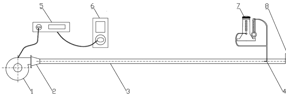
Fig. 1. Scheme of a measurement stand: 1– fan, 2 – confusor, 3 – measuring channel, 4 – Prandtl probe, 5 – fan’s operation regulator, 6 – wattmeter, 7 – compensation micro-manometer, 8 – flap valve [6]
