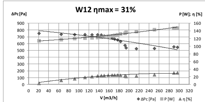
Fig. 13. Characteristics of fan W12
