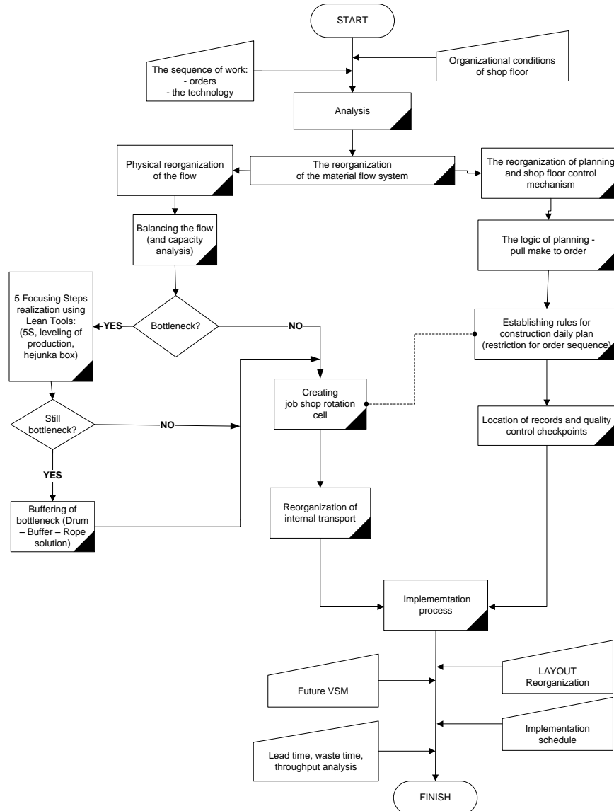
Fig. 3 General algorithm of the transformation unbalanced production unit (own study)
