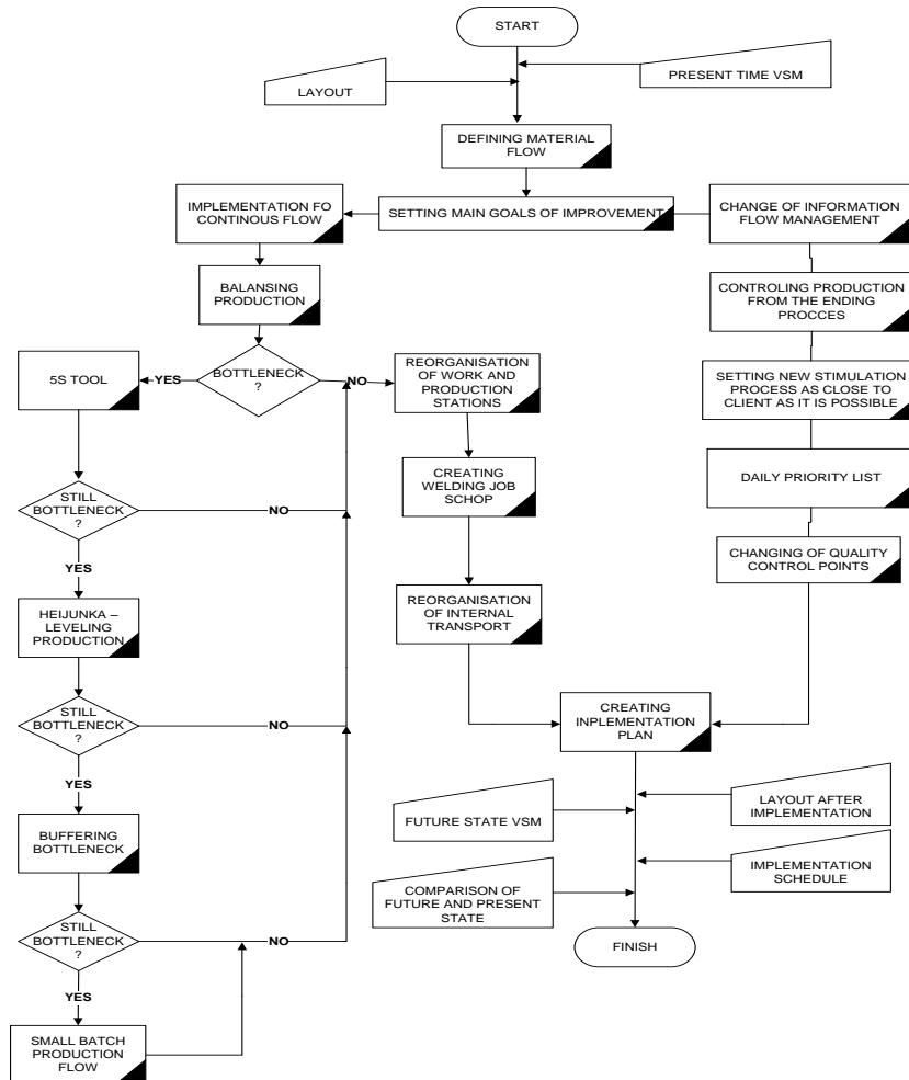
Fig. 2 Algorithm of optimization activities of production system (own study)
